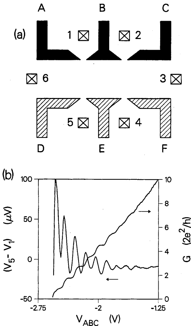
Fig. 1. (a) Schematic layout of the device used to demonstrate quantum oscillations in the thermopower of a QPC by means of a current heating technique. Hatched areas are gates, and crosses indicate Ohmic contacts. Black areas indicate gates whose voltage is varied in the experiment. The channel has a width of 4 \mu\text{m} and a length of 20 \mu\text{m} . (b) Measured conductance and transverse voltage ( V_5 - V_1 ) as a function of the gate voltage defining point contact 1 (black gates), at a lattice temperature of 1.65\text{K} and a current of 5 \mu\text{A} . The gates defining point contact 2 (dashed) were kept fixed at -2.0\text{V} .
