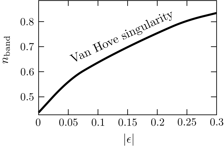
Figure 6.1. Band filling at which the dispersion relation (6.42) has a Van Hove singularity at the Fermi level, as a function of lattice distortion.
