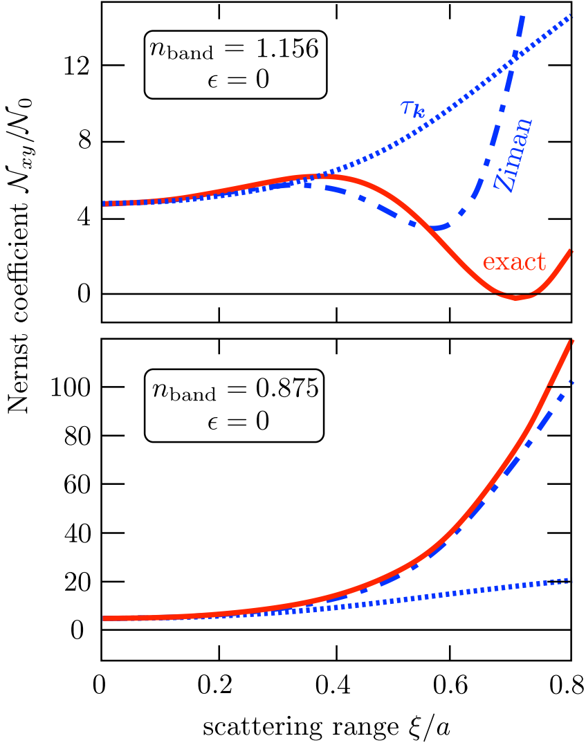
Figure 6.3. Dependence of the Nernst coefficient on the range \xi of the scattering potential, for an undistorted square lattice ( \epsilon = 0 ). Two values of the band filling are shown in the upper and lower panel. The three curves in each panel correspond to: the exact solution of the linearized Boltzmann equation (solid), the relaxation-time approximation (dotted), and Ziman's improvement on the relaxation-time approximation (dash-dotted).
