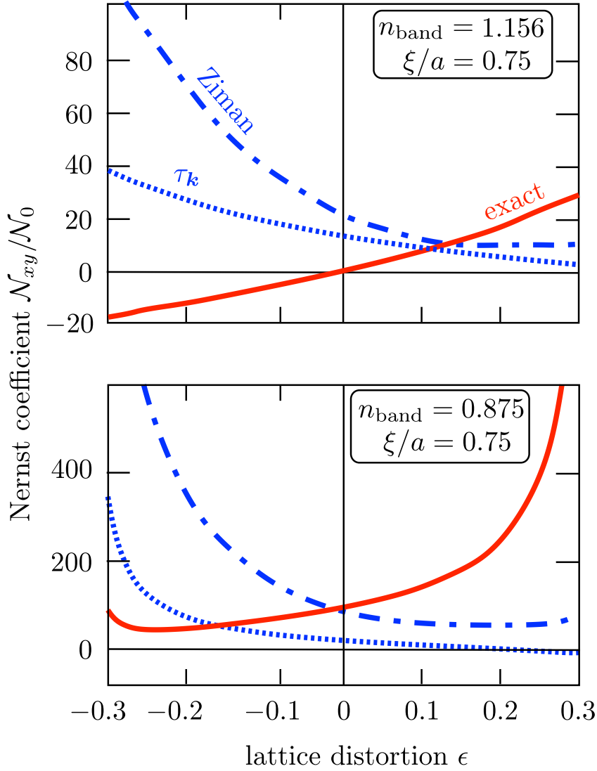
Figure 6.4. Same as Fig. 6.3, but now showing the dependence on the distortion \epsilon of the square lattice for a fixed range \xi = 0.75 a of the scattering potential.
