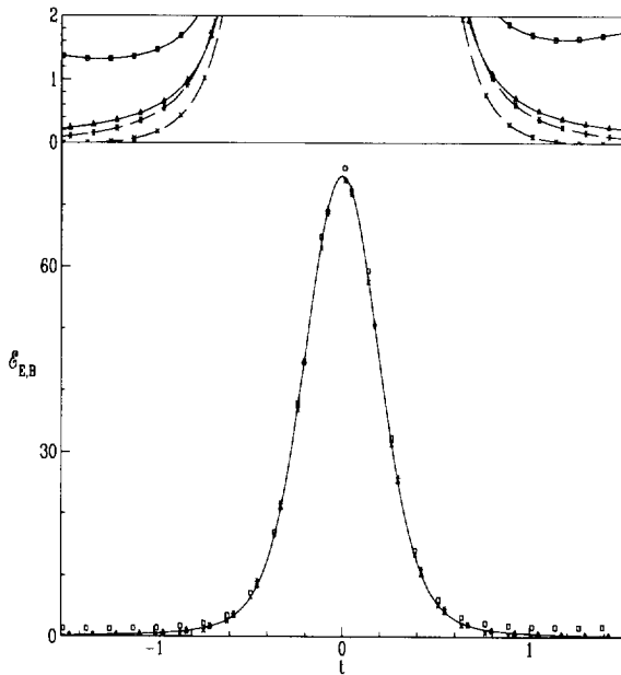
Figure 3. The electric and magnetic energies obtained after over-improved cooling for a lattice of spatial size N_s = 8 with boundary conditions fixed in the time direction to P_i = -1 at one and P_i = 1 at the other end [13]. Results are for N_t = 24 (squares for \mathcal{E}_E and crosses for \mathcal{E}_B , respectively the upper and lower curves in the inset) and N_t = 48 (triangles for \mathcal{E}_E and stars for \mathcal{E}_B , respectively the middle upper and lower curves in the inset).
