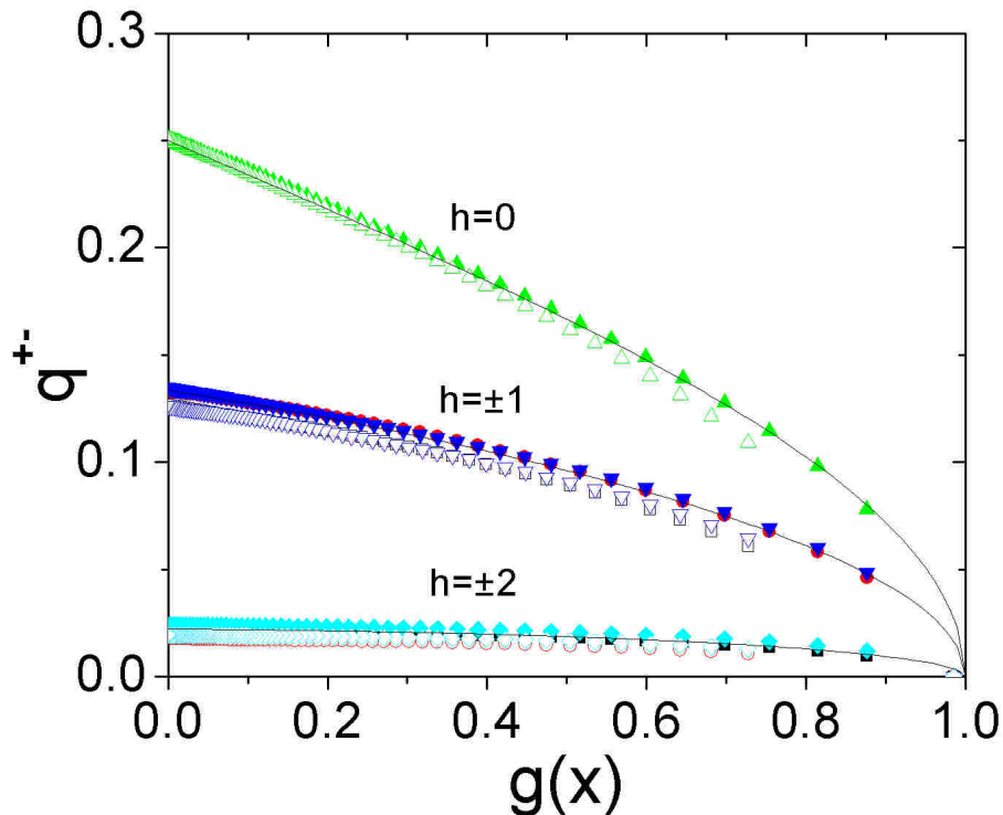
Figure 4: The function q^{+-}(h, g) as function of x through g = g(x, 0) , for some values of h (in units \langle h^2 \rangle^{1/2} ). The drawn lines are calculated and the points are the measured values.
