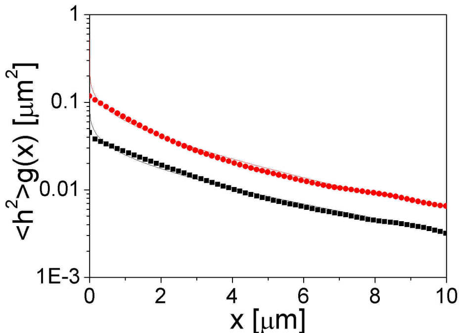
Figure 3: The spatial correlation function \langle h(x,0)h(0,0) \rangle for the statepoints II and IV fitted to the expression (10) using a cut-off.
