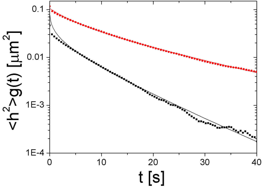
Figure 6: The correlation function \langle h(0, t)h(0, 0) \rangle . The points are experimental values and the lines curves according to (39) using a cut-off.
